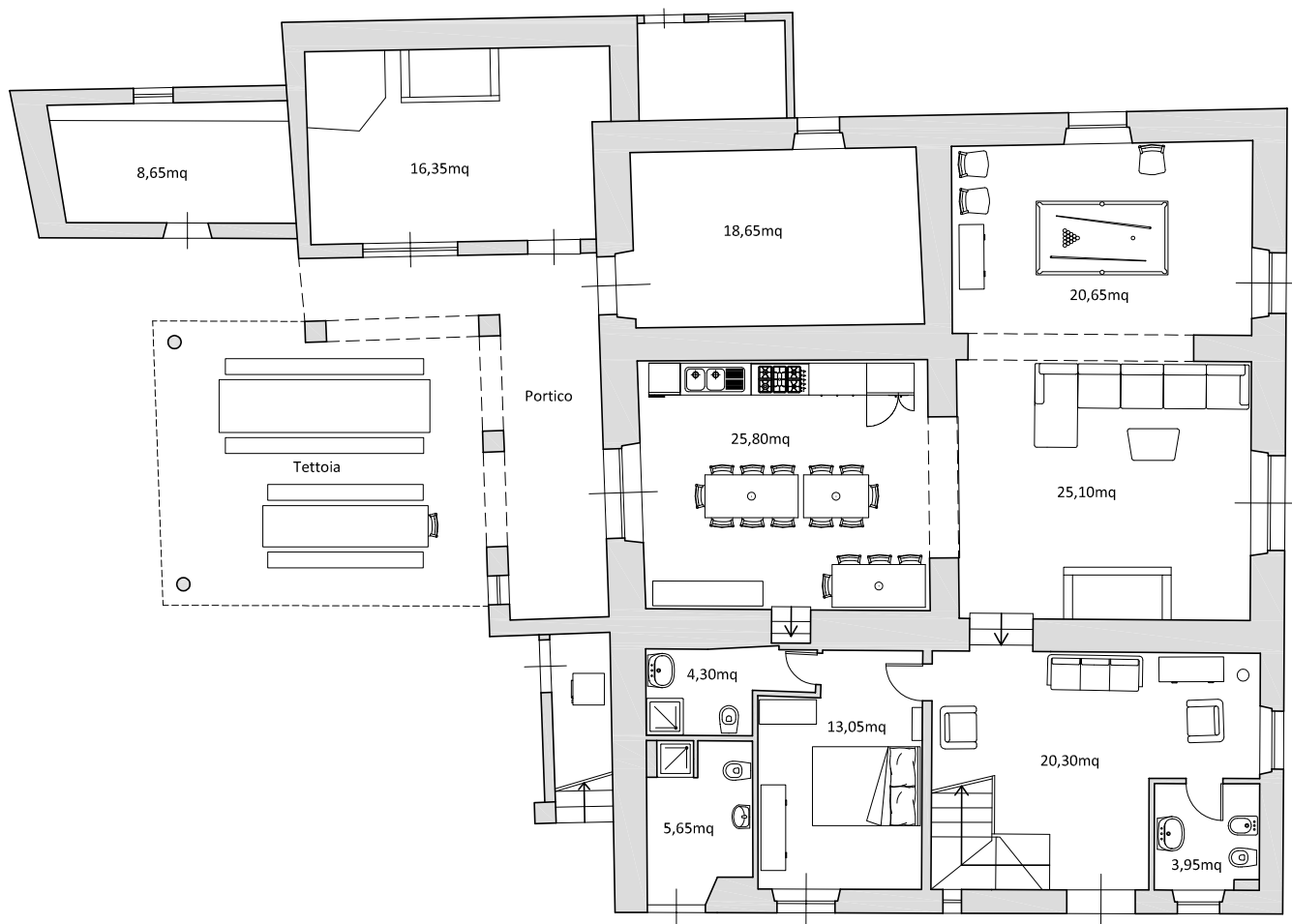
PIANO TERRA
